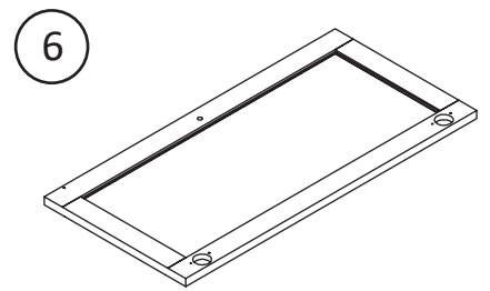
x1 T3969872060PK DOOR PANEL
