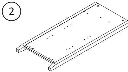
x1 T3969872020PK LEFT SIDE PANEL
