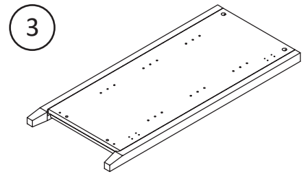
x1 T3969872030PK RIGHT SIDE PANEL
