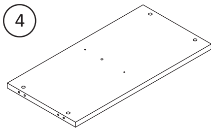
x1 T3969872040PK BOTTOM PANEL
